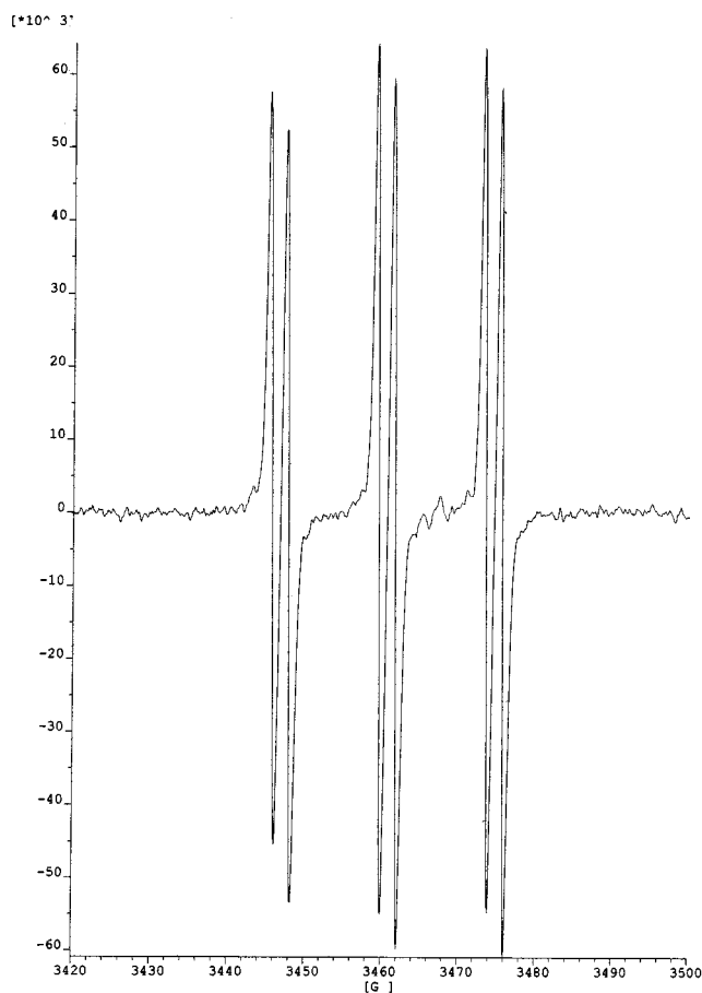
Figure 1. EPR spectrum obtained during irradiation ( \lambda > 320 nm) of an aerated cyclohexene/ \text{CH}_3\text{CN} (1:6 v/v) solution of \text{W}_{10}\text{O}_{32}^{4-} ( 1 \times 10^{-3} mol·dm ^{-3} ) in the presence of phenyl tert -butyl nitron ( 1 \times 10^{-3} mol·dm ^{-3} )
